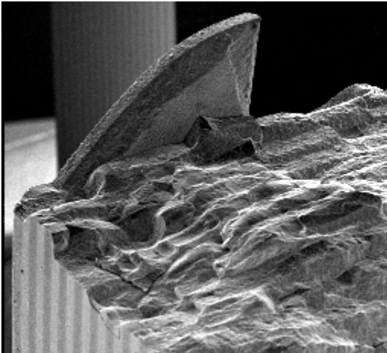
Fractured surface of an \text{Al}_2\text{O}_3\text{-ZrO}_2/\text{Al}_2\text{O}_3 laminate manufactured by tape casting. It has been demonstrated that certain types of laminates have an increased thermal shock resistance compared with the constituent layer materials.
